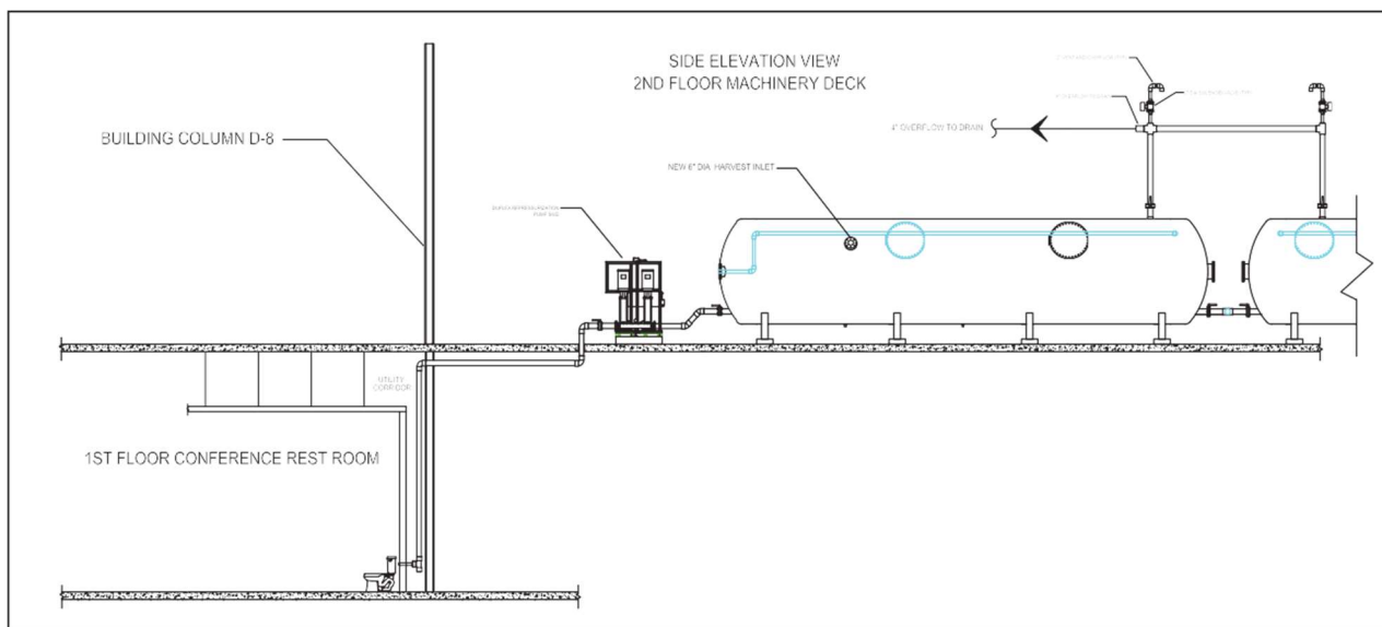
Plumbing Schematic
