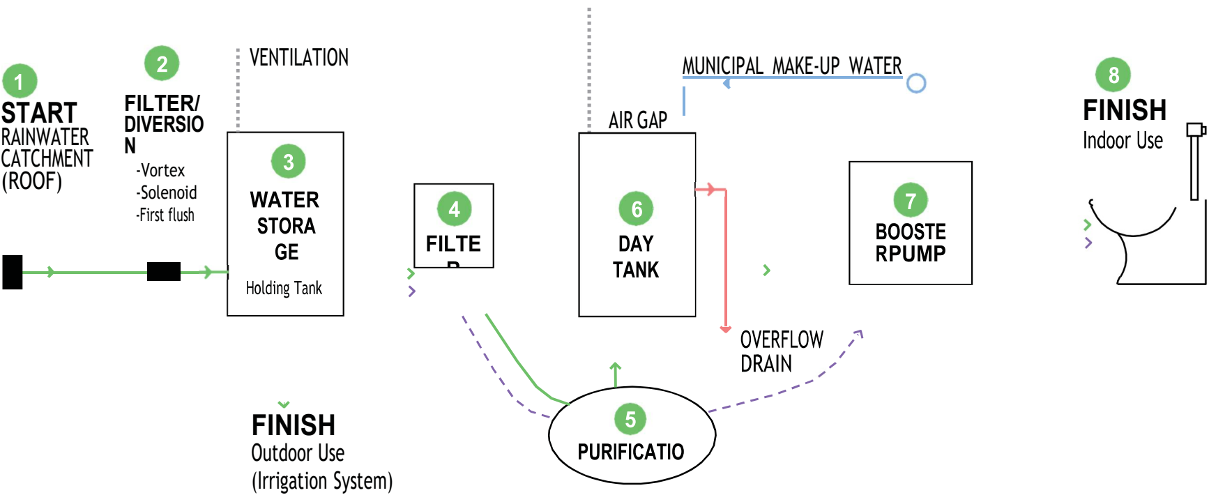
Sample Rainwater Harvesting System Diagram.
